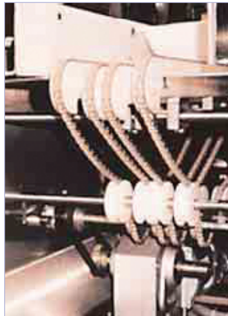
Rollers, sprockets and wearstrips manufactured from TIVAR® H.O.T. for applications in food processing show no signs of wear after numerous chemical and water washdowns, unlike their stainless steel counterparts.
