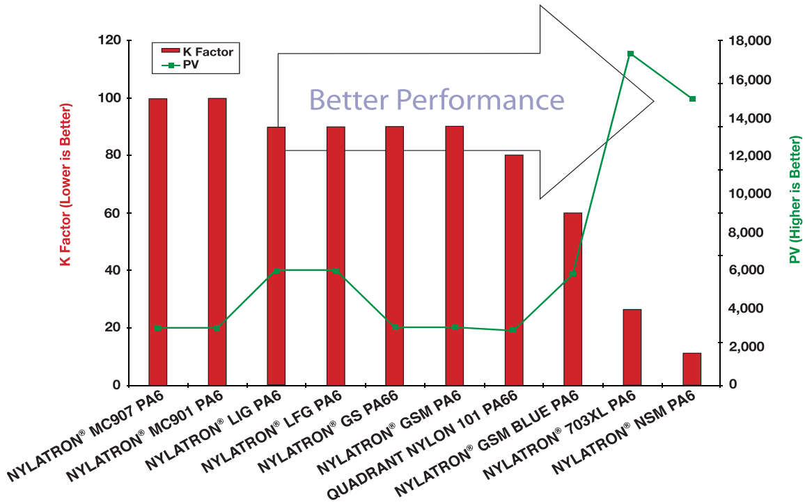
Fig.10 - WEAR RESISTANCE VS. LOAD BEARING CAPABILITY - NYLON MATERIALS
