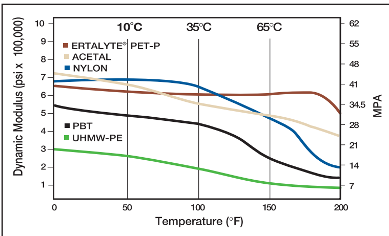
Fig. 13 - ERTALYTE® OFFERS BETTER STRENGTH IN HIGHER TEMPS
