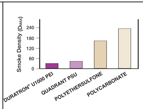
Fig. 20 - SMOKE EVOLUTION BY NBS TEST
