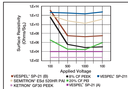
Fig. 33 - SURFACE RESISTIVITY
