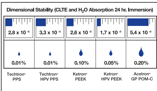
Fig. 25 - DIMENSIONAL STABILITY
