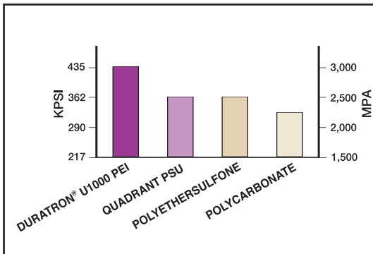
Fig. 19 - FLEXURAL MODULUS @ 73°F (23°C)
