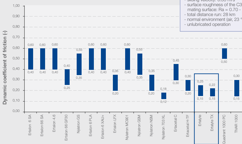
Fig. 1 Dynamic coefficient of friction (measured on a "plastics pin on rotating steel disk" - tribo system)
