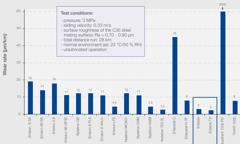
Fig. 2 Wear Resistance (measured on a "plastics pin on rotating steel disk" - tribo system)
